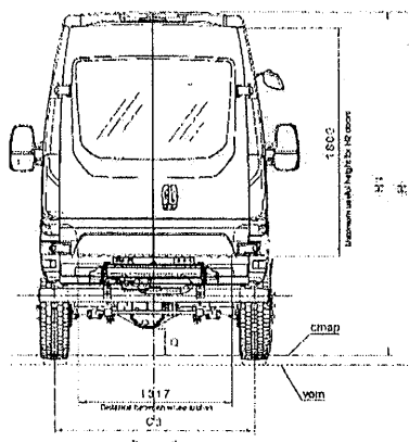
Rear view (Single wheels)
